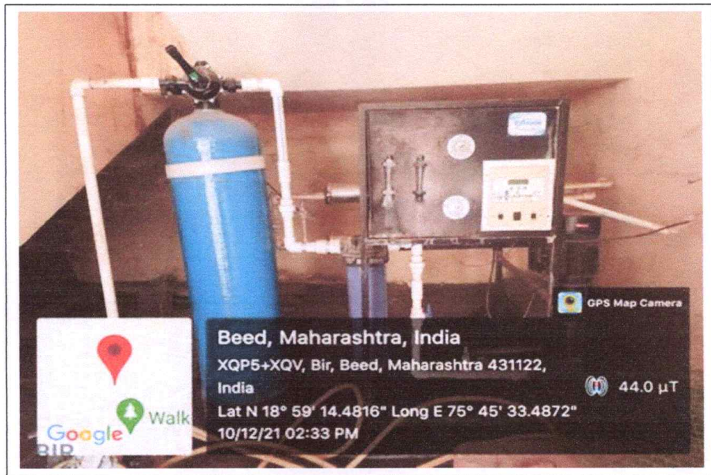
Central water purification RO system for minimum use of electricity and water wastage
